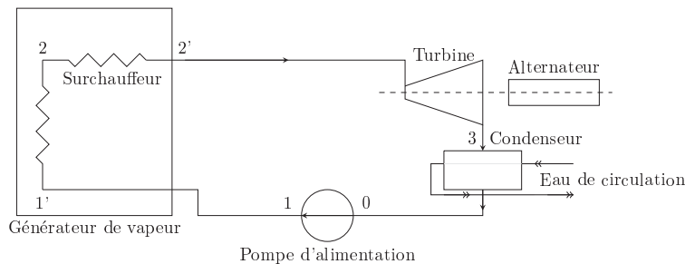
Figure 5 Cycle de Hirn.
