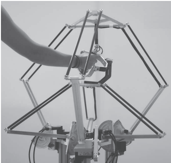
FIGURE 1 – Prototype du robot Delthaptic.
