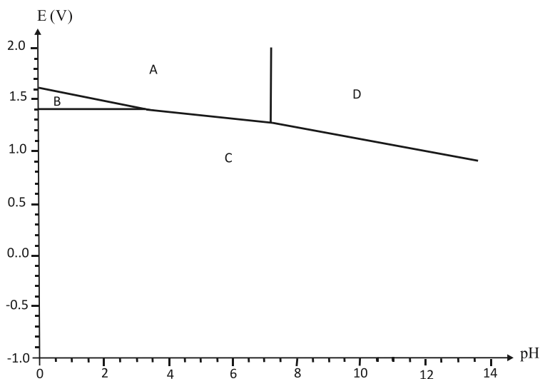
Figure 9 - Diagramme E-pH du chlore
