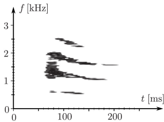
FIGURE 10 – Sonogramme du quetzal
